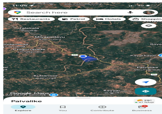
Map Screenshot
